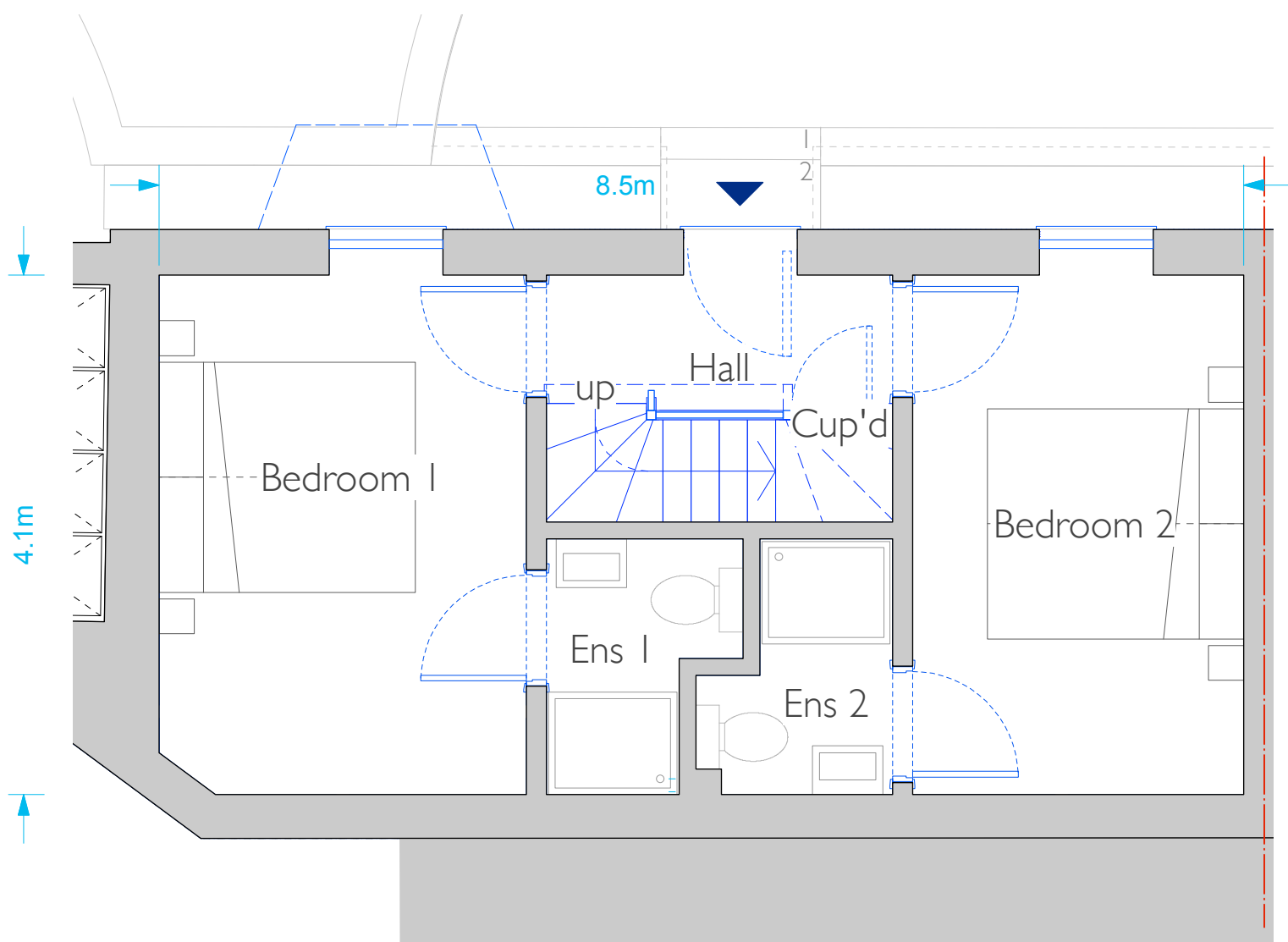
FIRST FLOOR
